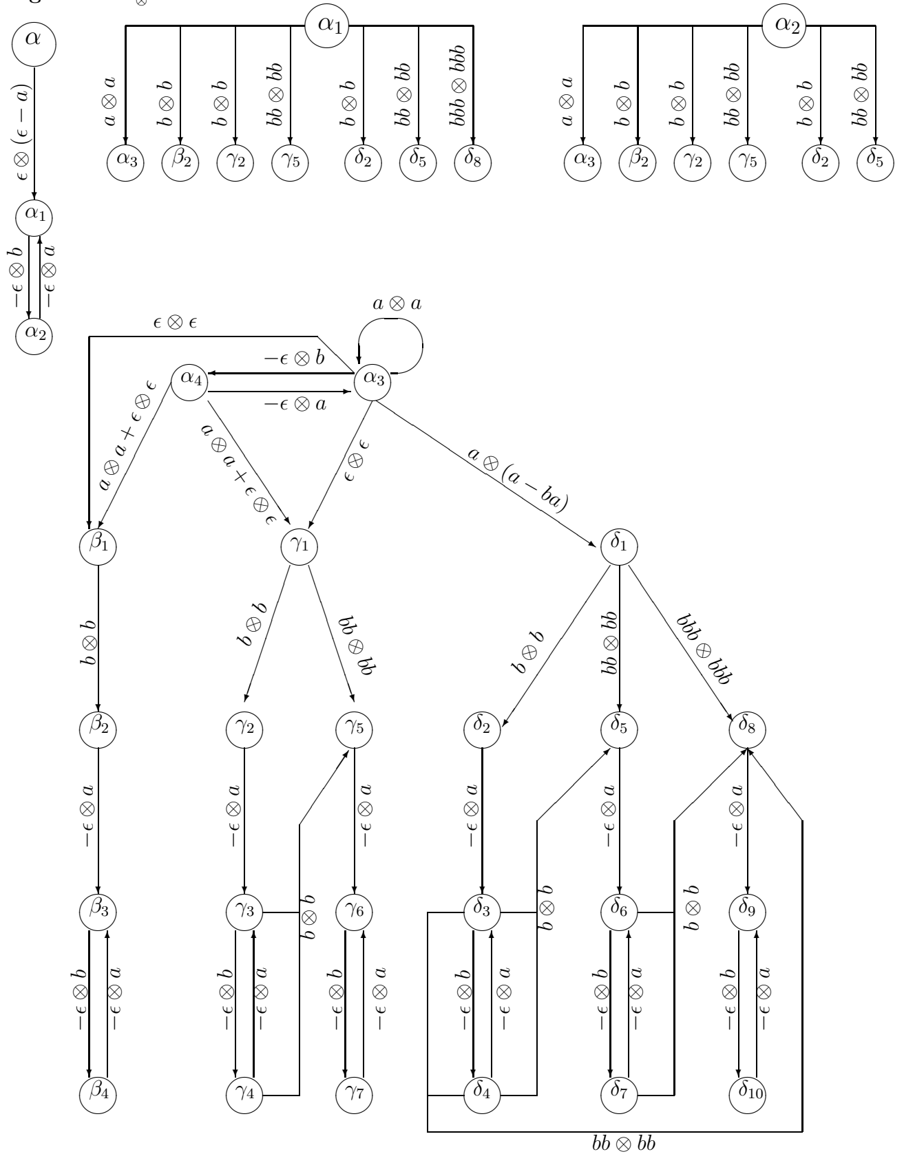
Figure 3: M_{\otimes}^3
